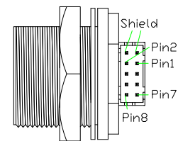
Pin Assignment
